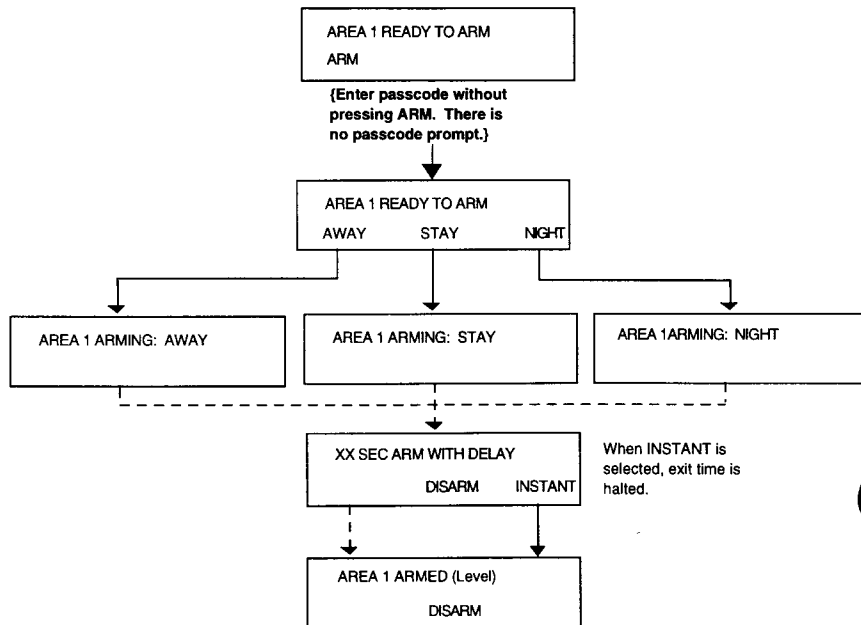
FIGURE 6 - QUICK ARMING
