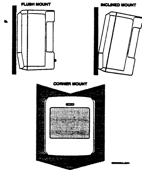
Figure 15. Wall Mount Options: use the inclined position for surface or corner mounting with the standard lens. Use the flush position for surface or corner mounting with the animal alley lens.
