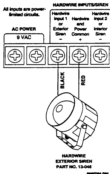
Figure 2. Exterior Siren Control Panel Connections
