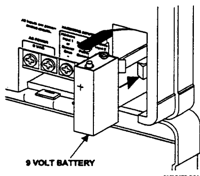
Figure 5. Control Panel Battery Installation
