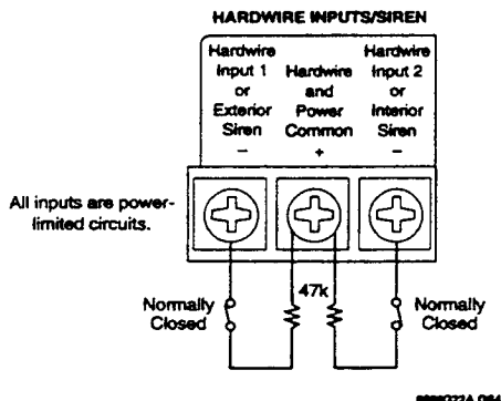
Figure 3. Wire Hardwire Sensors Normally Closed
